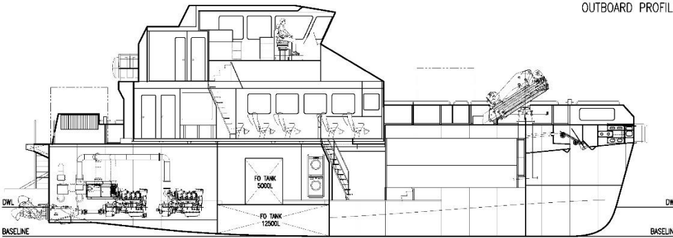
INBOARD PROFILE
